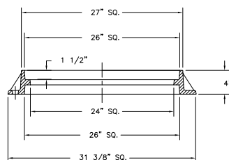
FRAME SECTION
