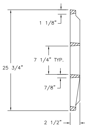
GRATE SECTION
