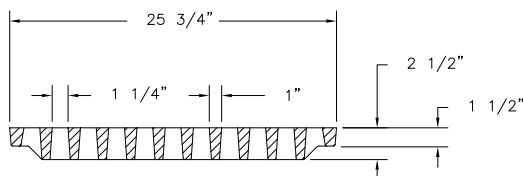
GRATE SECTION
